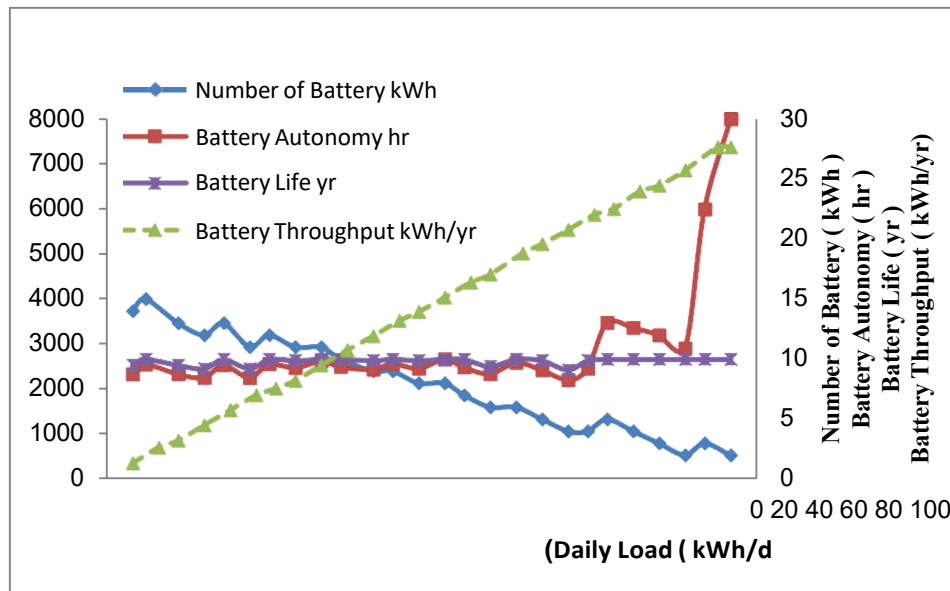
Fig. 3: Over the productivity of the battery, and the number of batteries, chargers self-battery, and the battery life time, compared with the daily load for the city of Baghdad.
