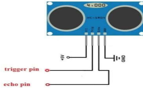
Figure 2: Pin diagram of ultrasonic sensor
