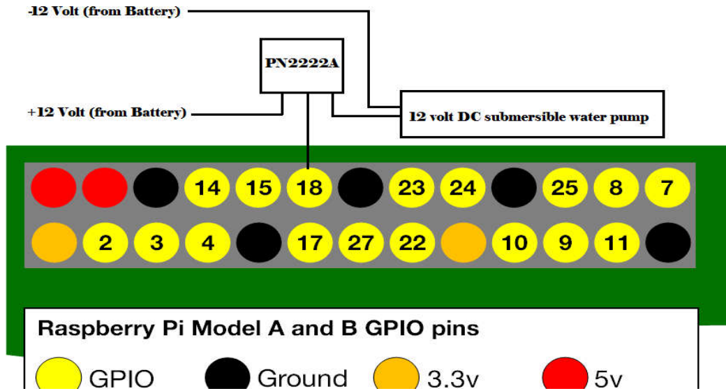
Figure 4: Connection diagram of 12 volt DC submersible water pump to Raspberry pi microcontroller
