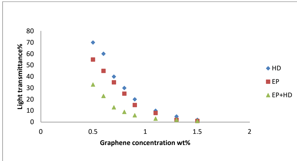
Light transmittance of graphene dispersion against graphene concentration
