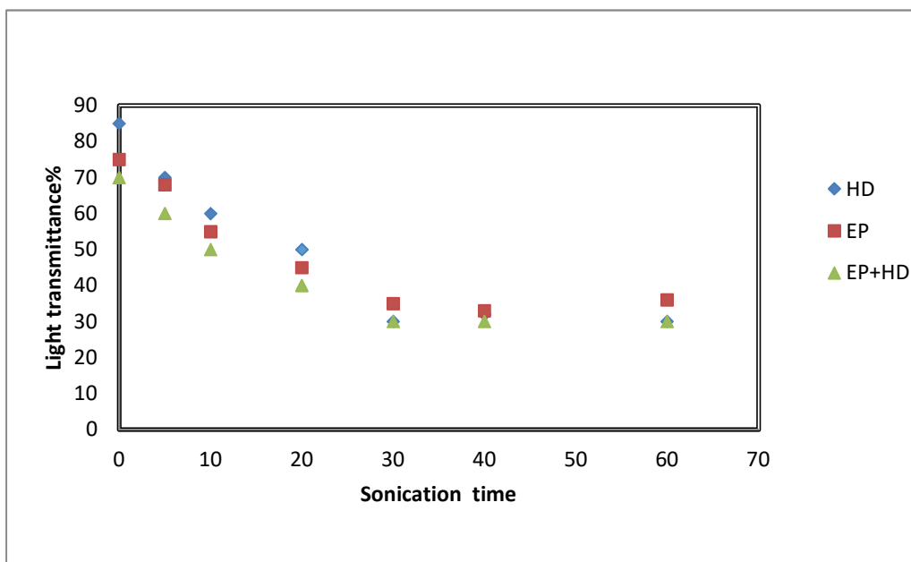
Light transmittance of graphene dispersion against sonication time (graphene concentration: 0.5 wt%).
